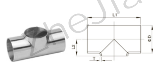
Short welded Tee AS No.XKKG-9061
