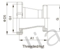
Threaded/nut
