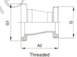
Threaded
