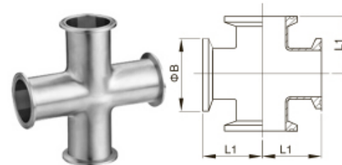
Clamped Cross BPE No.XK GK-9082
