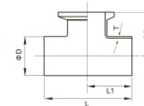
Single Outlet Tee Short Clip SMS No.XK GK-9021
