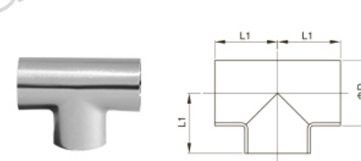
Short welded Tee 3A No.XK GK-9033
