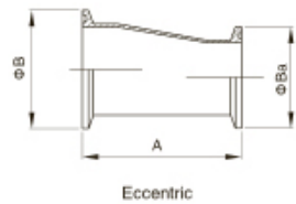
Eccentric
